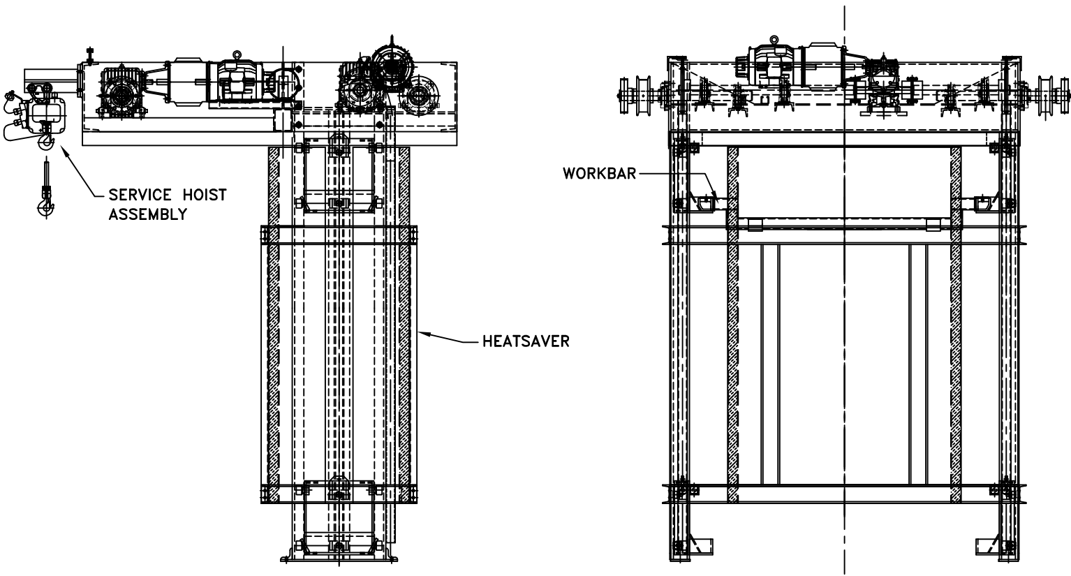
UPTON MIGHTYMATIC AUTOMATED HOIST ASSEMBLY U-HOIST
