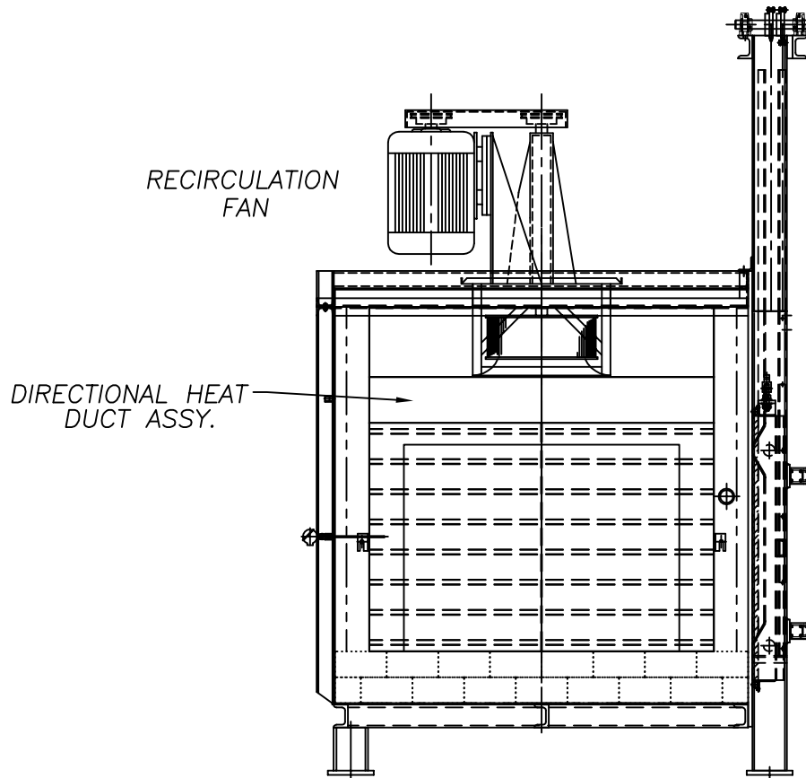
UPTON BOX TYPE FURNACE U-BE
