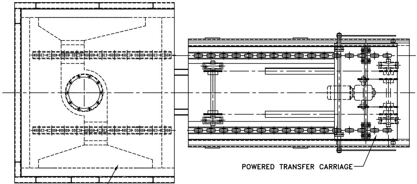
DIRECTIONAL HEAT DUCT ASSY.
