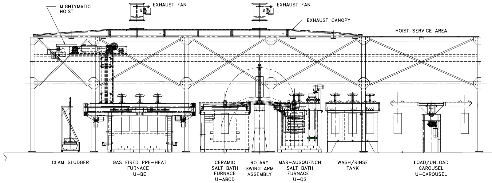
UPTON AUTOMATED SALT BATH FURNACE SYSTEM
