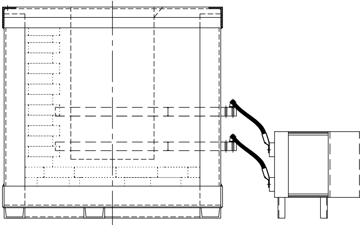
SUBMERGED ALLOY ELECTRODE SALT BATH FURNACE CERAMIC TYPE SALT BATH FURNACE U-ABCD
